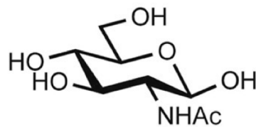
N -Acetyl-D-glucosamine (GlcNAc)
